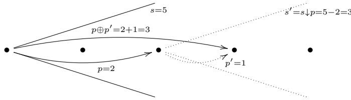
Fig. 2. The “template” of non-empty lists of shape 5 (length 6)
